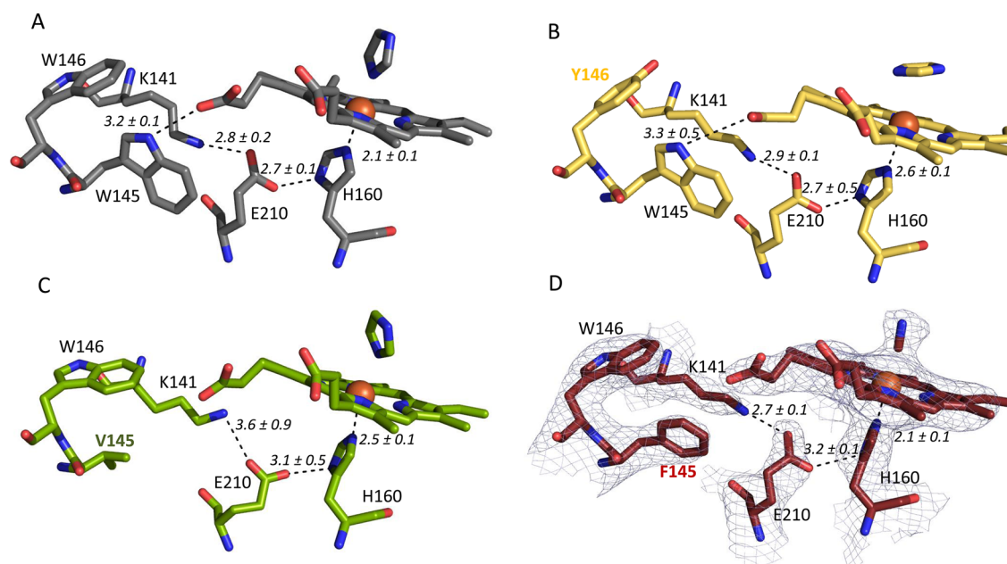
Figure 2. Architecture of the proximal heme side of wild-type NdCld (A) and the variants W146Y (B), W145V (C) and W145F (D) together with its 2F_o - |F_c| electron density map countered at 1\sigma level (D). Figures were generated using PyMOL ( http://www.pymol.org/ ). Putative H-bonds are shown as dotted black lines.
